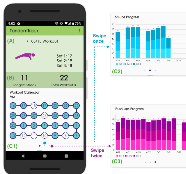
Figure 2. The home screen of the TandemTrack mobile app: the daily exercise feedback (A); a summary of the longest streak and complete exercise sessions (B); a series of aggregated feedback—exercise streak view (C1), sit-up performance (C2), and push-up performance (C3).
